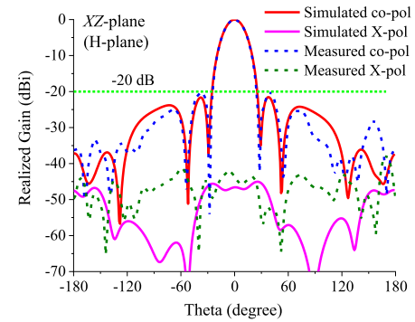
Fig. 17. Simulated and measured patterns at 3.44GHz: (a) XZ-plane and (b) YZ-plane.
