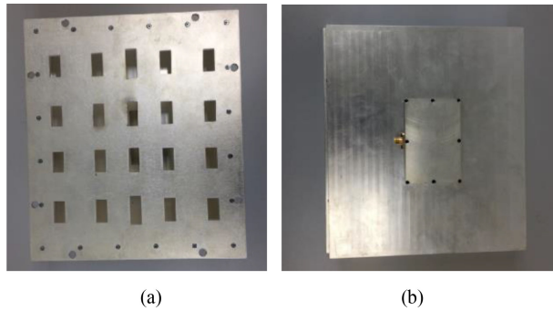
Fig. 15. Photographs of the proposed 5 \times 4 antenna array : (a) Top view and (b) Bottom view.
